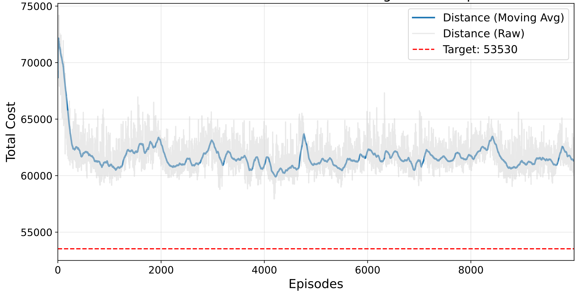
Final Masked AutoRL-SOP Training - ft70.4.sop
